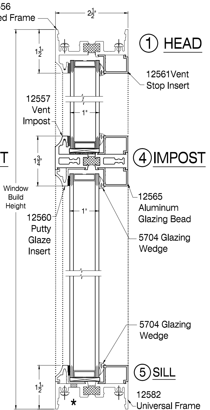
VERTICAL SECTION
