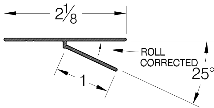
FLANGE EXTENDER #5807
