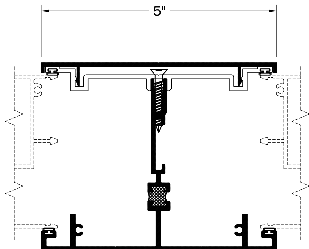
3 1/4" THREE PIECE STRUCTURAL MULLION
