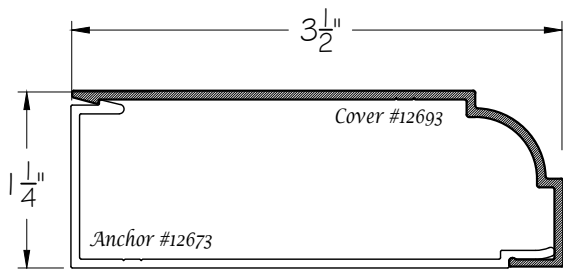
3 1/2" x 1 1/4" (AB)
