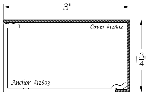
3" x 1 3/4" (S)
