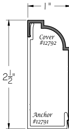
1" x 2 1/2" (AC)
