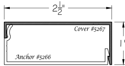
1" x 2 1/2" (C)
