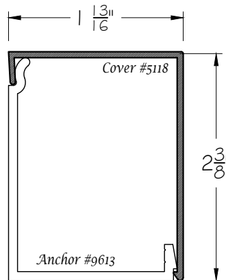
1 13/16" x 2 3/8" (E)
