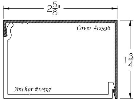
1 3/4" x 2 5/8" (W)
