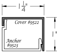
1" x 1 1/4" (A)
