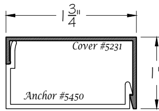
1" x 1 3/4" (B)
