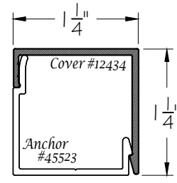
1 1/4" x 1 1/4" (F)
