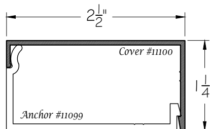
1 1/4" x 2 1/2" (H)
