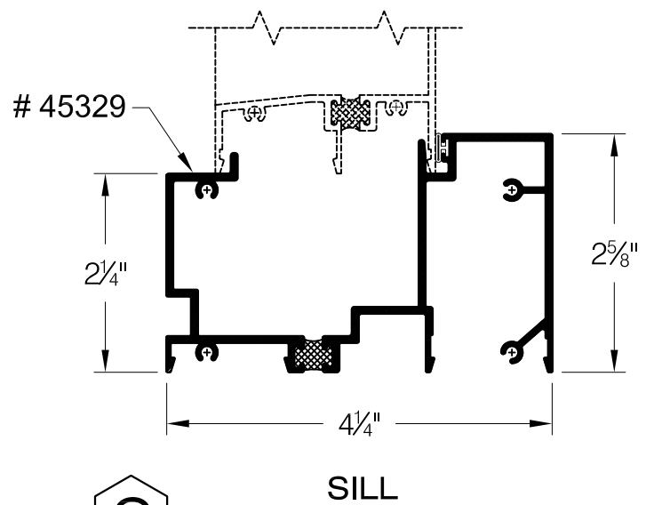
10# Framemaster Subsill
